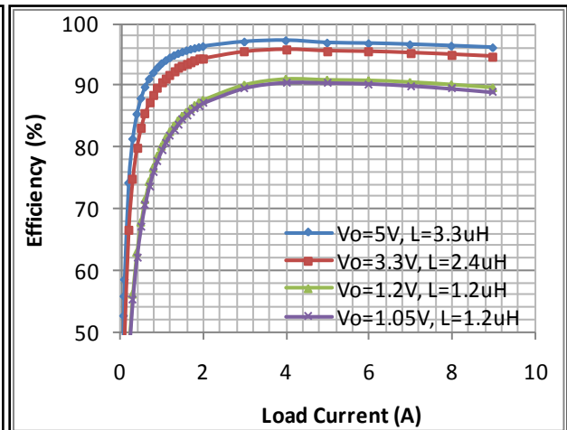
Figure 9. FAN23SV06PA Efficiency vs. Load Current with V_{IN}=12\text{ V} and f_{SW}=500\text{ kHz}
