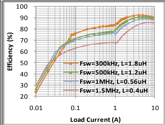
Figure 7. FAN23SV06A Efficiency vs. Load Current with V_{IN}=12\text{ V} and V_{OUT}=1.2\text{ V}
