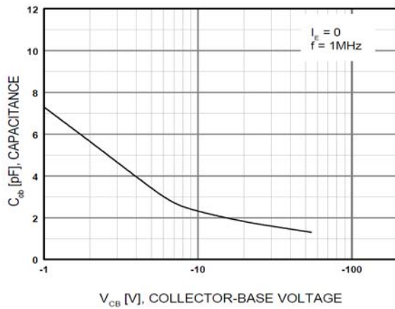
Figure 3. Output Capacitance
