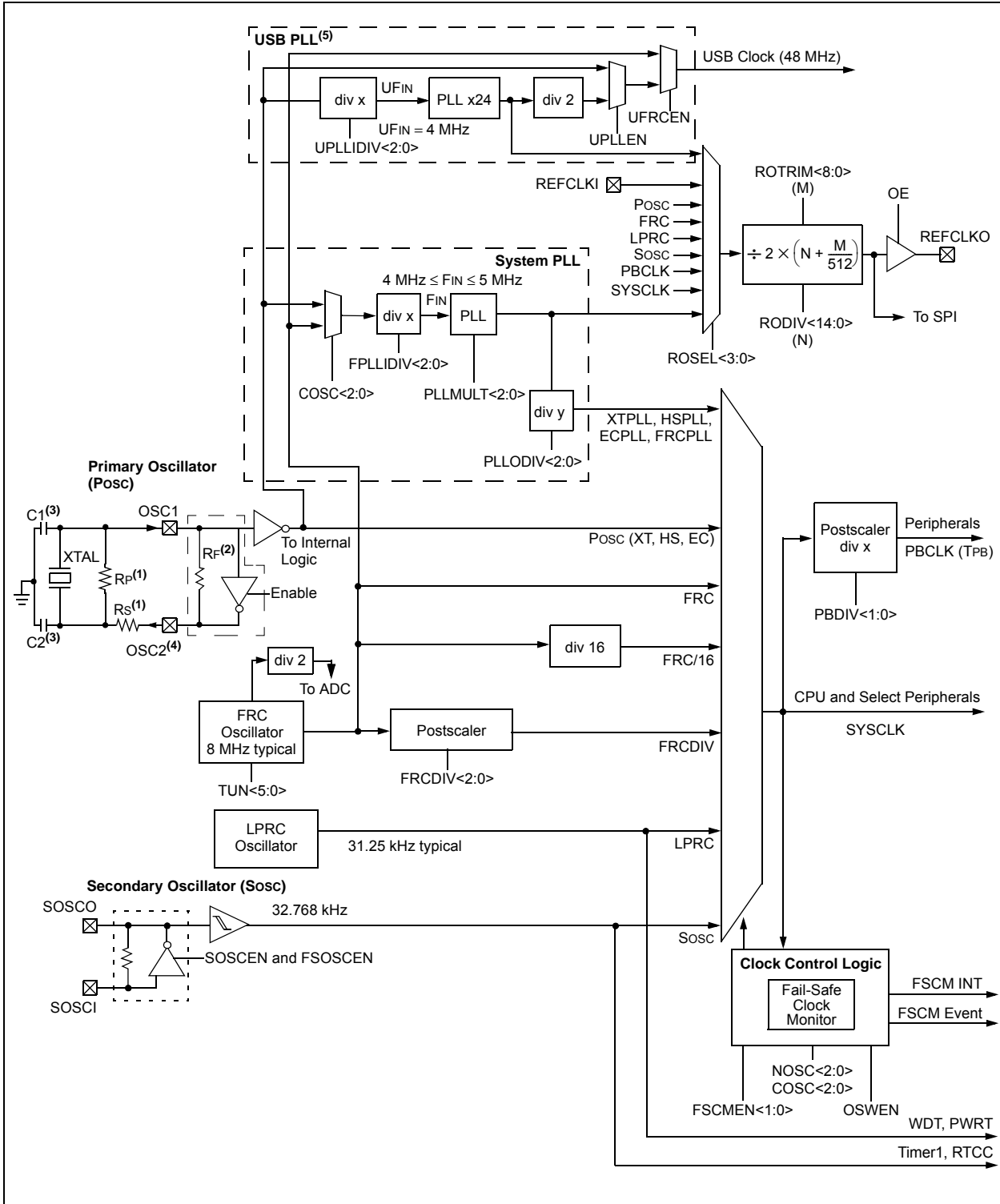
FIGURE 8-1: OSCILLATOR DIAGRAM
