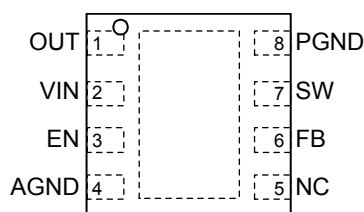
8-Pin 2mm x 2mm MLF ® (ML) (Top View)
