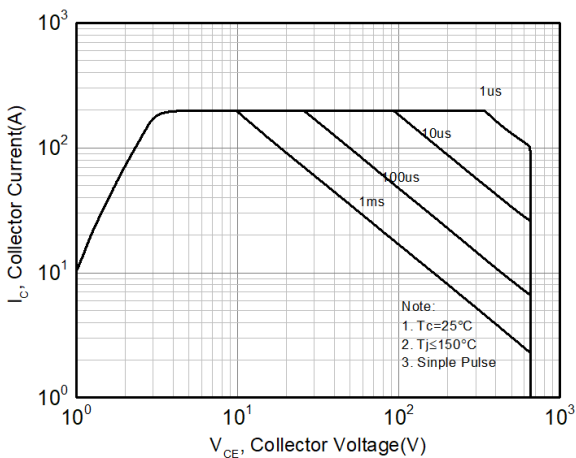
Figure 17. FBSOA
