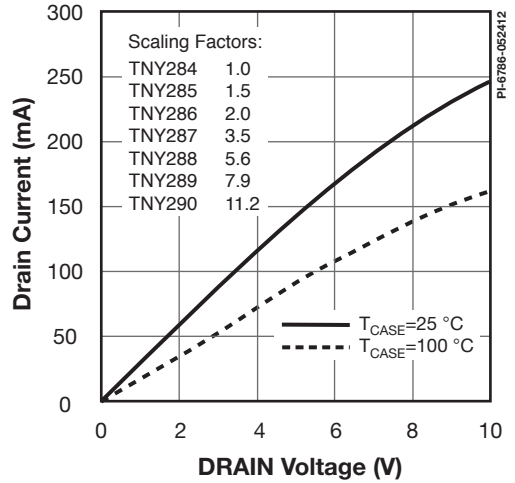
Figure 26. Output Characteristic.
