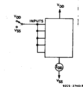
Fig. 17 — Quiescent device current test circuit.
