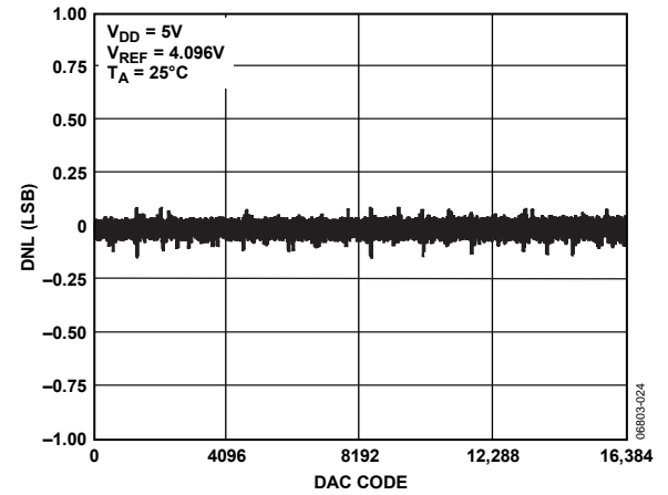
Figure 13. AD5024 DNL
