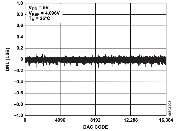
Figure 12. AD5044 DNL
