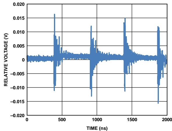
Figure 29. Digital Feedthrough
