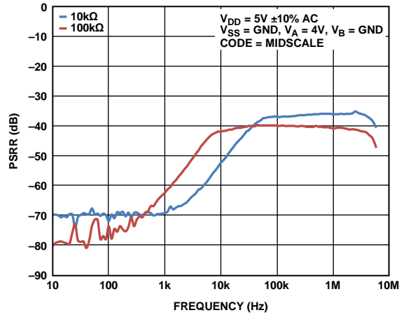
Figure 28. Power Supply Rejection Ratio (PSRR) vs. Frequency
