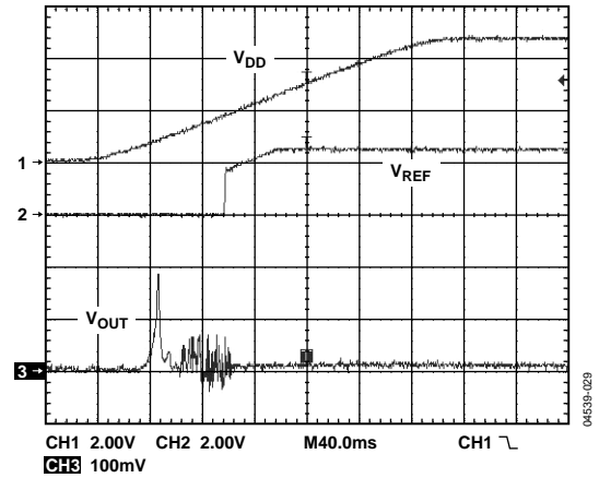
Figure 28. Power-On Reset to 0 V—AD5660-2
