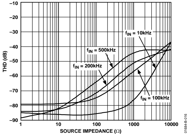
Figure 16. THD vs. Source Impedance for Various Analog Input Frequencies
