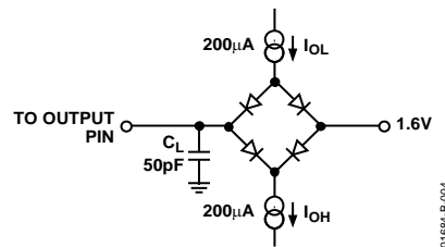
Figure 4. Load Circuit for Digital Output Timing Specifications
