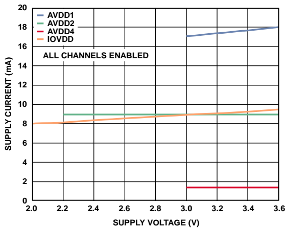
Figure 69. Supply Current vs. Supply Voltage at 8 kSPS, High Resolution Mode
