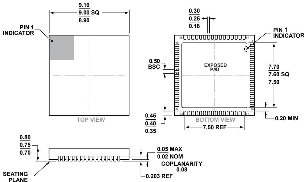
Figure 122. 64-Lead Lead Frame Chip Scale Package [LFCSP] 9 mm x 9 mm Body and 0.75 mm Package Height (CP-64-15)
