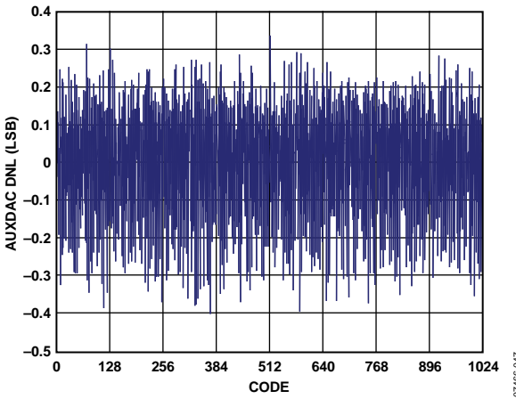
Figure 79. AD9114/AD9115/AD9116/AD9117 AUXDAC DNL
