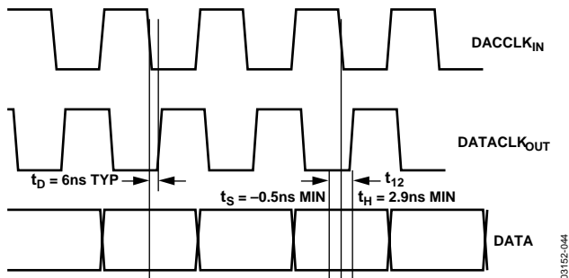
Figure 44. Data Timing, 1x Interpolation, DCLKPOL = 0
