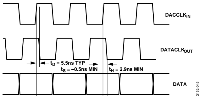
Figure 45. Data Timing, 1x Interpolation, DCLKPOL = 1
