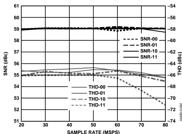
Figure 82. SNR and THD Performance vs. f_{ADC} and SPGA Bias Setting with RxPGA = 0 dB, f_{IN} = 10 MHz, LPF set to 26 MHz, and AIN = -1 dBFS
