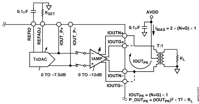
Figure 64. Current-Mode Operation
