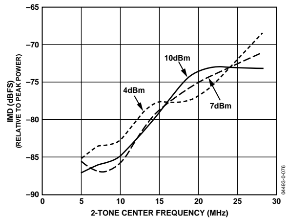
Figure 31. 2-Tone IMD Frequency Sweep vs. Peak Power with f_{DATA} = 80 MSPS, 2 \times Interpolation
