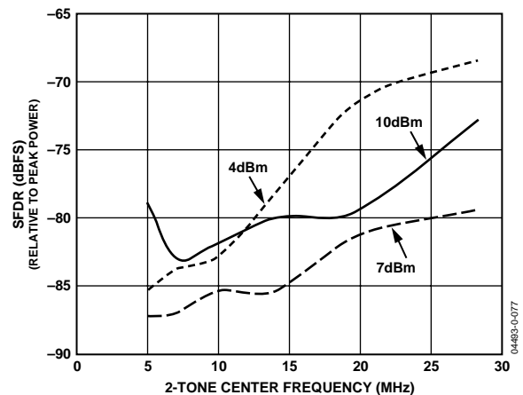
Figure 32. 2-Tone Worst Spur Frequency Sweep vs. Peak Power with f_{DATA} = 80 MSPS, 2 \times Interpolation
