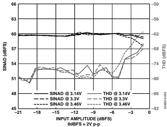
Figure 5. SINAD and THD vs. Input Amplitude and Supply ( f_{IN} = 8 MHz, LPF f_{-3dB} = 26 MHz; Rx PGA = 0 dB)
