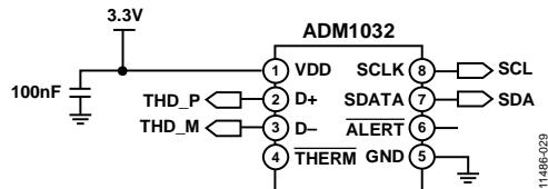
Figure 26. Example External Temperature Sensor Circuit
