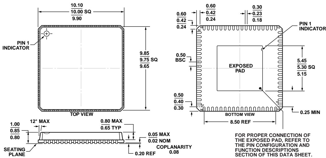
Figure 91. 72-Lead Lead Frame Chip Scale Package [LFCSP_VQ] 10 mm × 10 mm Body, Very Thin Quad (CP-72-6) Dimensions shown in millimeters
