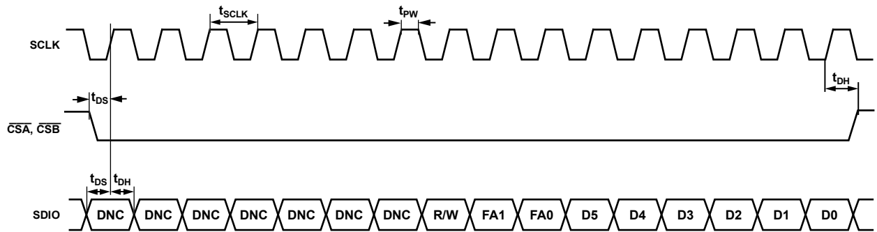
Figure 52. SPI Interface Read/Write Mode Timing Diagram
