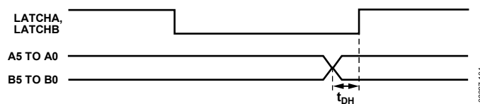
Figure 4. Parallel Mode Timing Diagram
