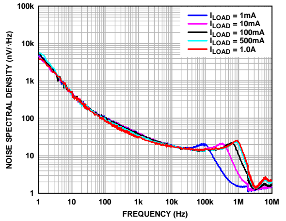
Figure 44. Output Noise Spectral Density, Adjustable Version, V_{OUT} = 1.2 V
