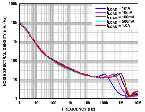
Figure 45. Output Noise Spectral Density, V_{OUT} = 3 V
