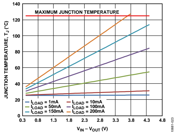
Figure 23. TSOT 500 mm 2 of PCB Copper, T A = 25°C
