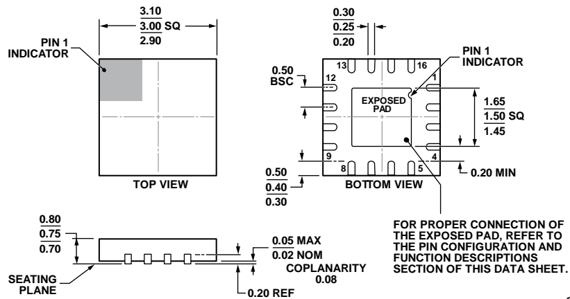
Figure 64. 16-Lead Lead Frame Chip Scale Package [LFCSP_WQ] 3 mm × 3 mm Body, Very, Very Thin Quad (CP-16-27) Dimensions shown in millimeters
