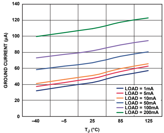
Figure 14. Ground Current vs. Junction Temperature, Single Output Loaded, V_{RIPPLE} = 50\text{ mV} , C_{OUT} = 1\ \mu\text{F}
