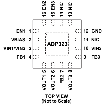
Figure 4. ADP323 Pin Configuration
