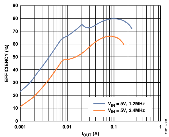
Figure 8. Efficiency vs. Current Load ( I_{OUT} ), V_{IN} = 5V , V_{OUT} = -30V , T_A = 25^\circ\text{C}
