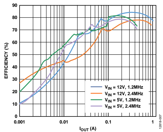
Figure 7. Efficiency vs. Current Load ( I_{OUT} ), V_{IN} = 5V and 12V , V_{OUT} = -15V , T_A = 25^\circ\text{C}
