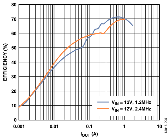
Figure 5. Efficiency vs. Current Load ( I_{OUT} ), V_{IN} = 12V , V_{OUT} = -2.5V , T_A = 25^\circ\text{C}
