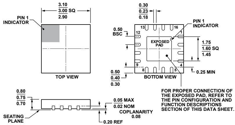
Figure 27. 16-Lead Lead Frame Chip Scale Package [LFCS] 3 mm × 3 mm Body and 0.75 mm Package Height (CP-16-22)
