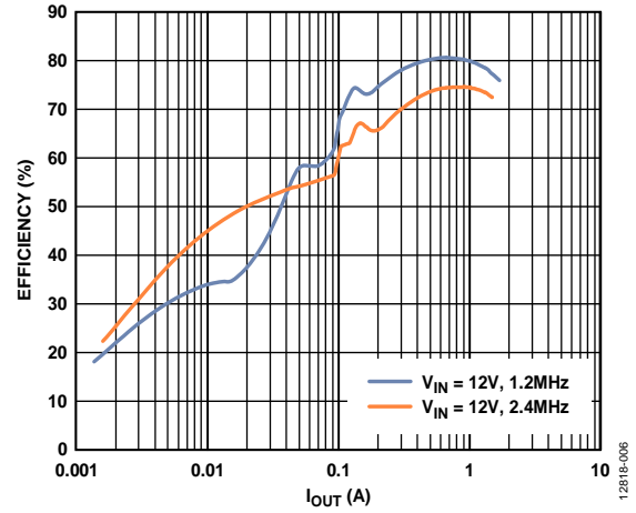
Figure 6. Efficiency vs. Current Load ( I_{OUT} ), V_{IN} = 12V , V_{OUT} = -5V , T_A = 25^\circ\text{C}
