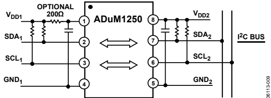
Figure 9. Typical Isolated \text{I}^2\text{C} Interface Using the ADuM1250
