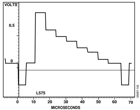
Figure 141. PAL Chroma
