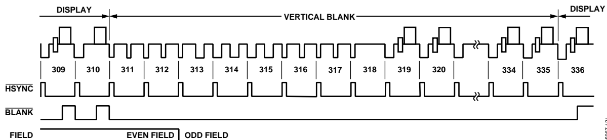
Figure 121. SD Timing Mode 3 (PAL)
