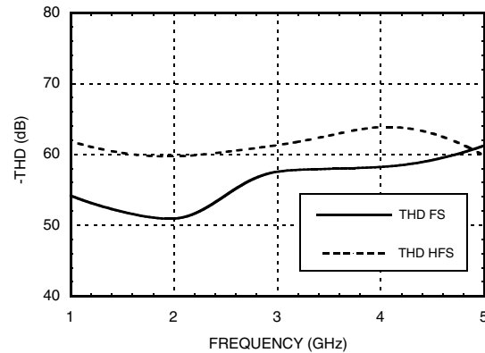
Hold-Mode THD vs. Frequency & Input Power @ f_{clk} = 4 GHz @ 0 dBm
