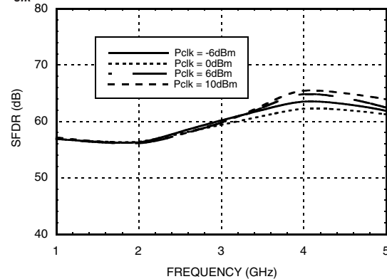
Hold-Mode SFDR vs. Frequency & Clock Power @ Full Scale Input Level (1 Vp-p), f_{clk} = 1 GHz Sinusoid
