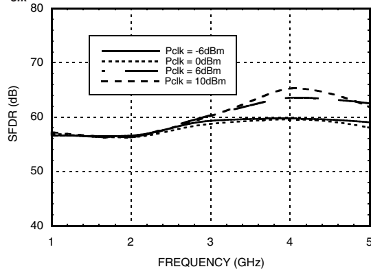
Hold-Mode SFDR vs. Frequency & Clock Power @ Full Scale Input Level (1 Vp-p), f_{clk} = 500 MHz Sinusoid
