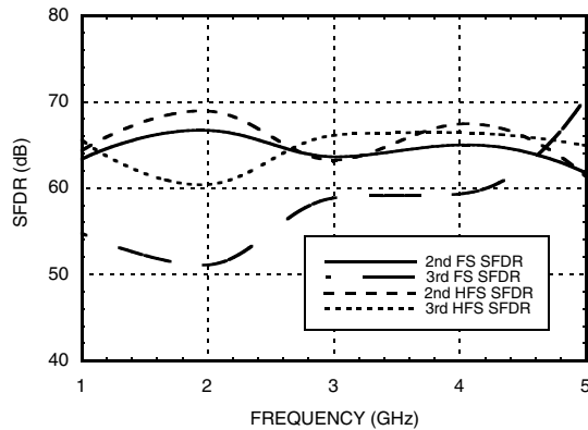
Hold-Mode SFDR vs. Frequency & Input Power @ f_{clk} = 4 GHz @ 0 dBm
