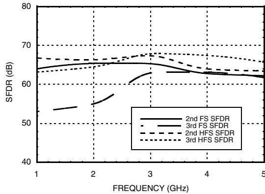
Hold-Mode SFDR vs. Frequency & Input Power @ f_{clk} = 3 GHz @ 0 dBm
