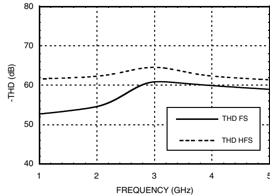
Hold-Mode THD vs. Frequency & Input Power @ f_{clk} = 3 GHz @ 0 dBm
