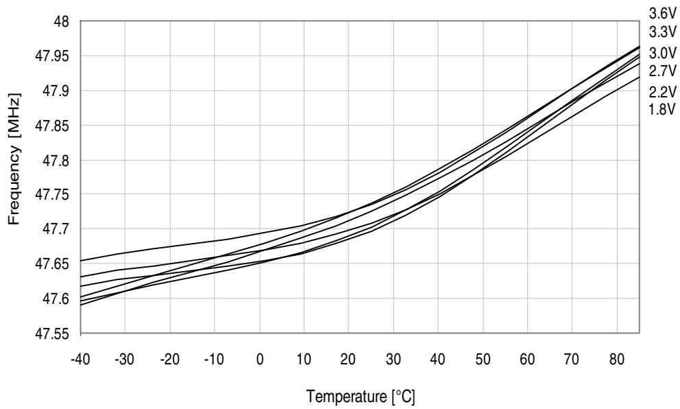
Figure 33-317. 48MHz internal oscillator frequency vs. temperature.
