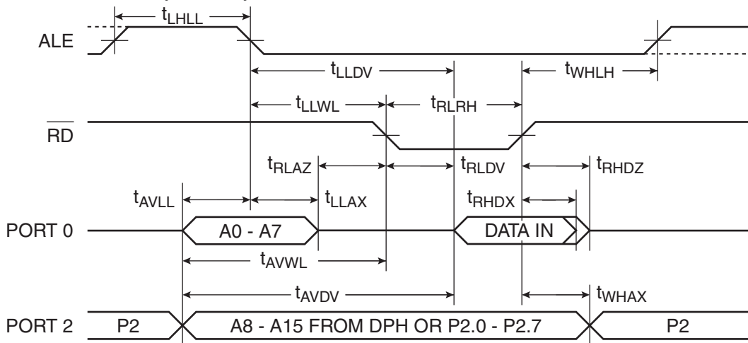
Figure 18-15. External Data Memory Read Cycle
