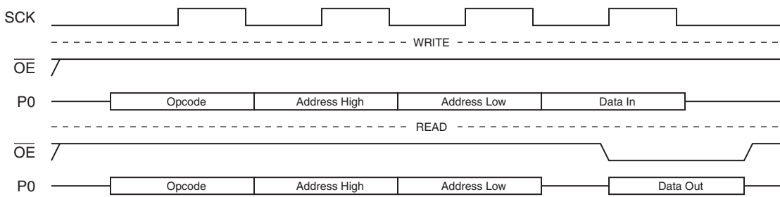
Figure 17-7. ISP Command Packet (Parallel Byte)
