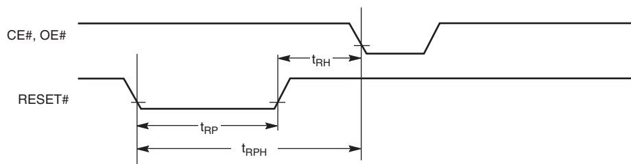
Figure 10.10 Reset Timings
