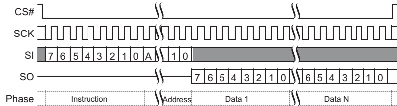
Figure 9.27 Read Command Sequence (3-Byte Address, 03h or 13h)
