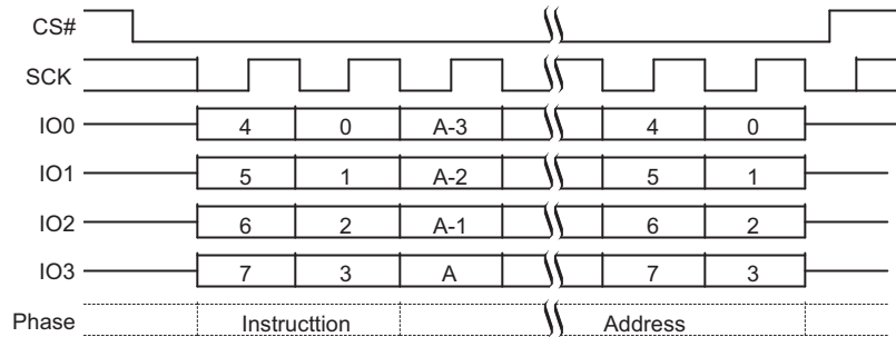
Figure 9.46 Parameter Sector Erase (P4E 20h or 4P4E 21h) QPI Mode Command Sequence
