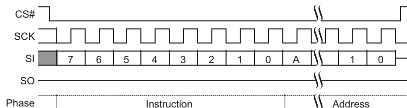
Figure 9.47 Sector Erase (SE D8h or 4SE DCh) Command Sequence
