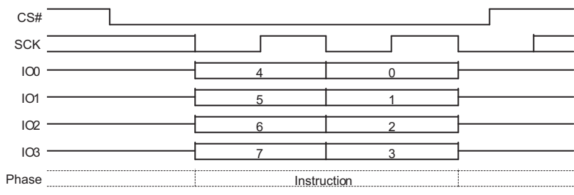
Figure 9.16 Write Disable (WRDI) Command Sequence QPI Mode
