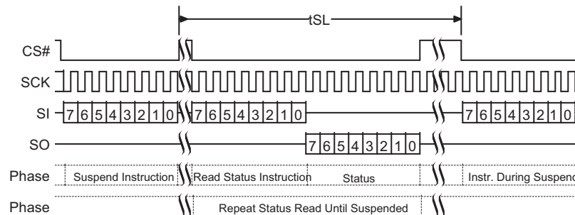
Figure 9.53 Program or Erase Suspend Command Sequence
