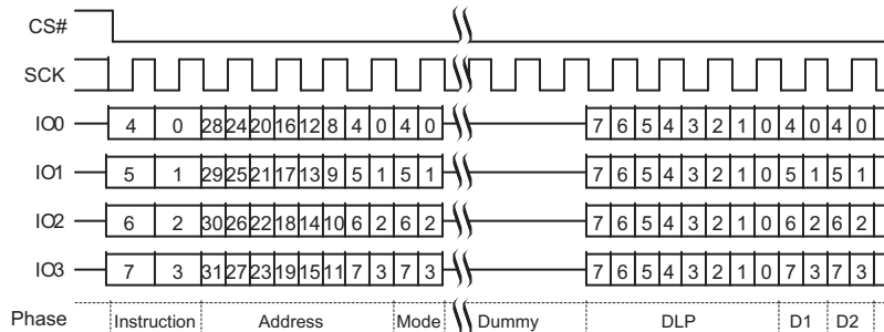
Figure 9.41 DDR Quad I/O Read Initial Access (4-Byte Address, EEh or EDh [CR2V[7]=1]) QPI Mode
