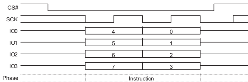
Figure 9.75 Mode Bit Reset Command Sequence QPI Mode
