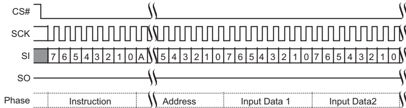
Figure 9.43 Page Program (PP 02h or 4PP 12h) Command Sequence
