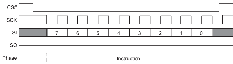
Figure 9.15 Write Disable (WRDI) Command Sequence
