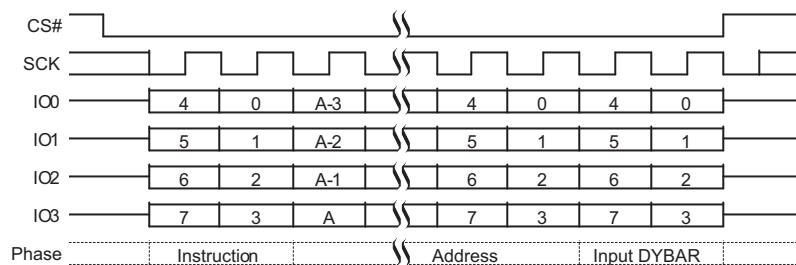
Figure 9.62 DYBWR Command Sequence
