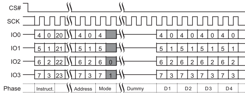
Figure 9.33 Quad I/O Read Command Sequence (3-Byte Address, EBh [CR2V[7]=0]) QPI Mode
