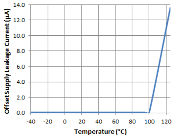
Figure 27. Offset Supply Leakage Current vs. Temperature
