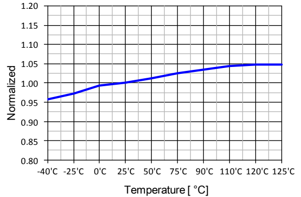
Figure 9. Shutdown Delay Current ( I_{DELAY} ) vs. T_A .
