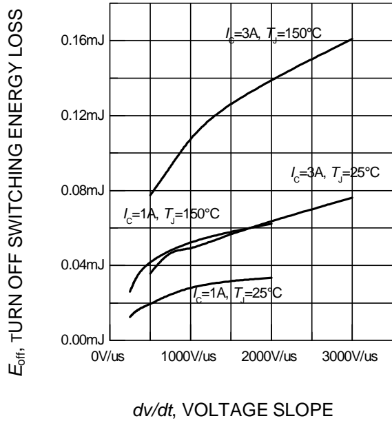
dv/dt , VOLTAGE SLOPE Figure 16. Typical turn off switching energy loss for soft switching (dynamic test circuit in Fig. E)
