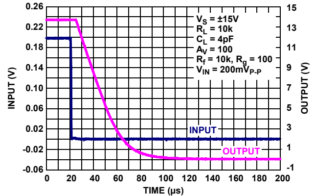
FIGURE 52. POSITIVE OUTPUT OVERLOAD RESPONSE TIME, V_S = \pm 15V
