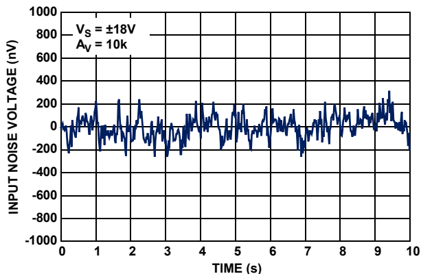
FIGURE 53. INPUT NOISE VOLTAGE 0.1Hz TO 10Hz, V_S = \pm 18V
