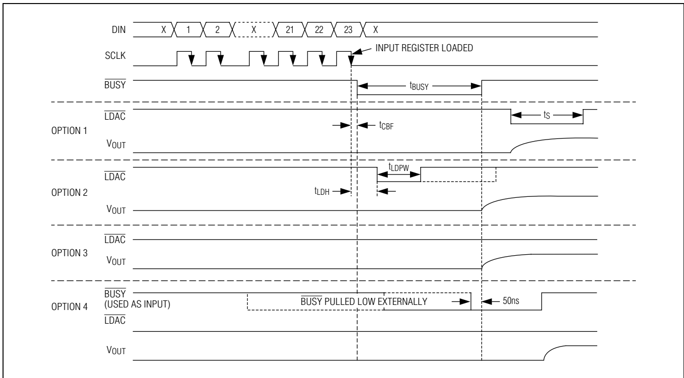
Figure 4. \text{BUSY} and \overline{\text{LDAC}} Timing
