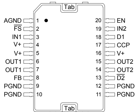
Figure 3. 33887 Pin Connections
