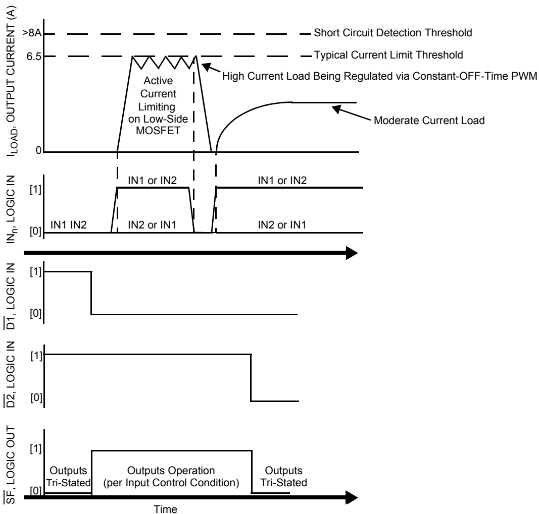
Figure 10. Operating States
