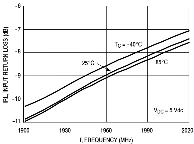
Figure 17. Input Return Loss (S11) versus Frequency
