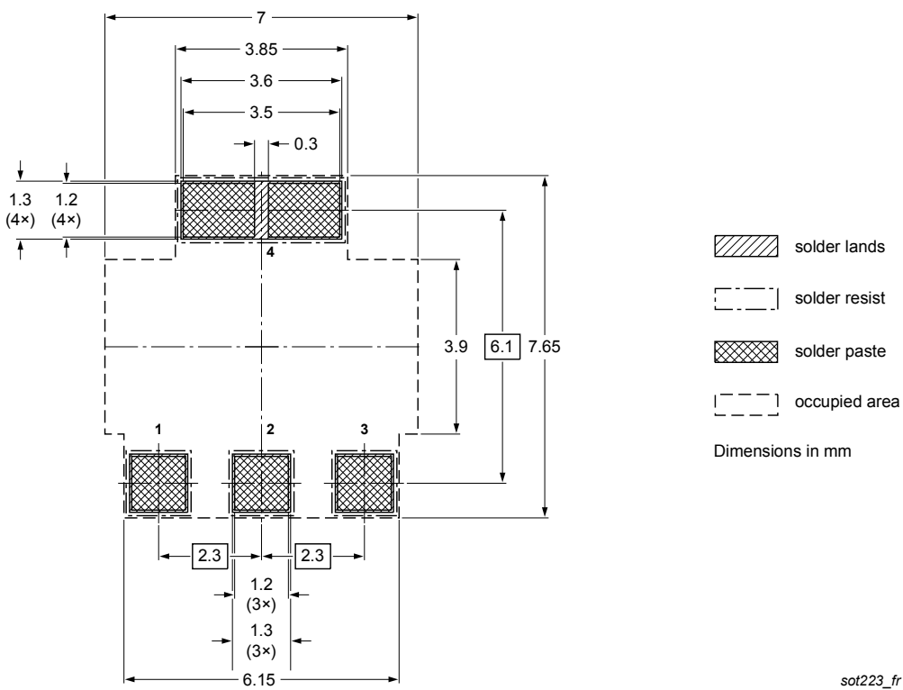
Fig. 14. Reflow soldering footprint for SC-73 (SOT223)
