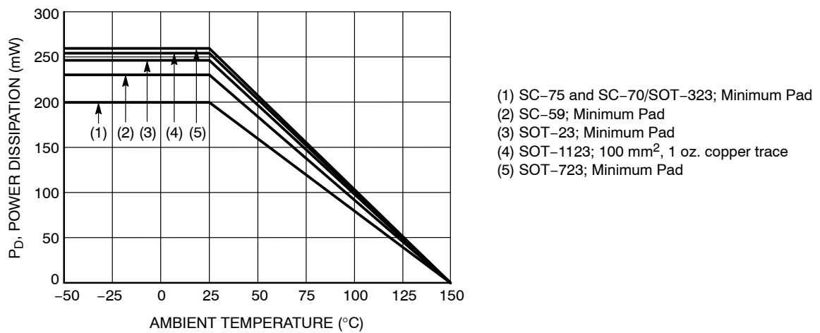
Figure 1. Derating Curve
