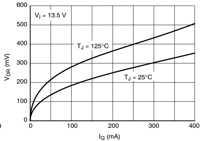
Figure 11. Drop Voltage vs. Output Current
