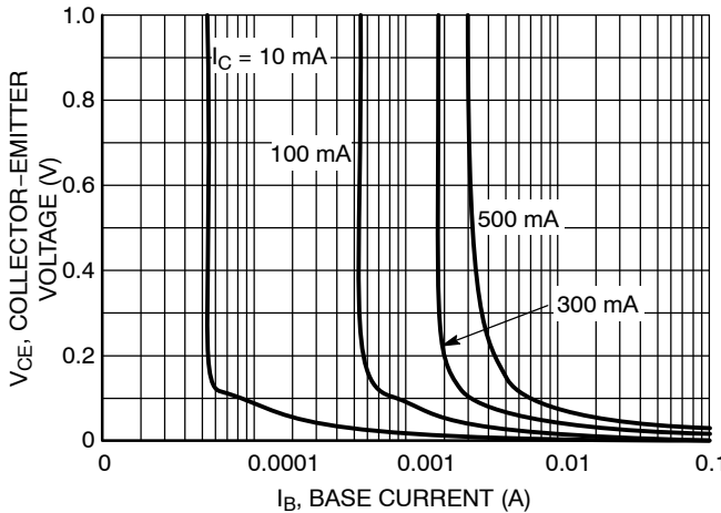
Figure 5. Saturation Region
