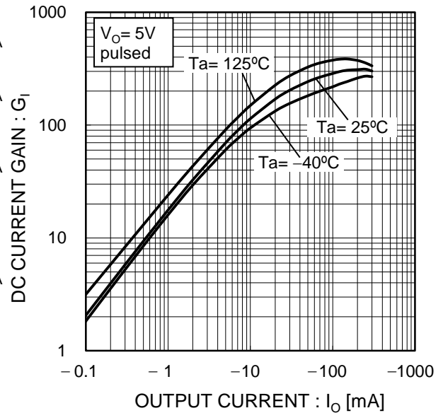
Fig.4 DC current gain vs. output current
