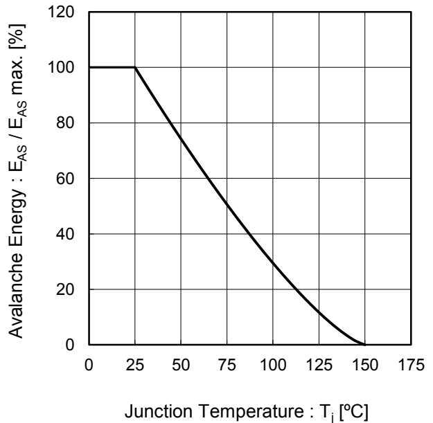
Fig.4 Avalanche Energy Derating Curve vs Junction Temperature
