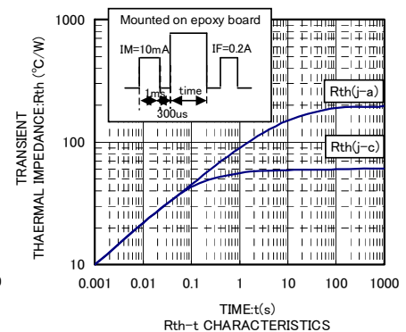
Rth-t CHARACTERISTICS
