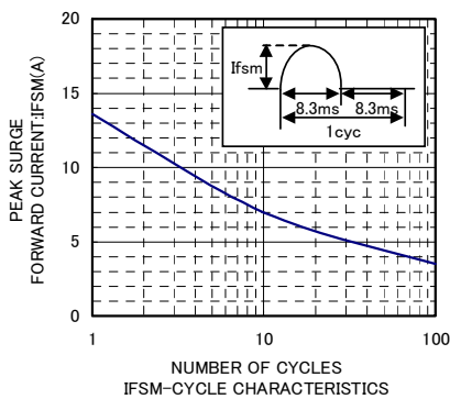
IFSM-CYCLE CHARACTERISTICS
