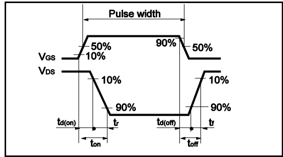
Fig.1-2 Switching Waveforms
