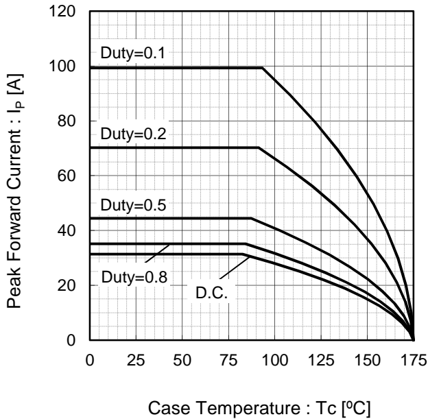
Fig.7 I_p - T_c Derating Curve
