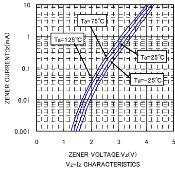
V_z - I_z CHARACTERISTICS
