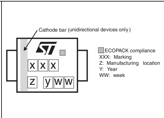
Figure 24. Marking layout (1)
