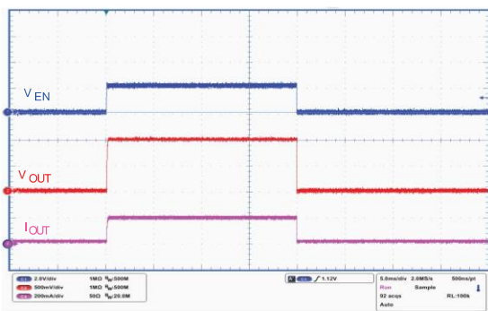
Figure 18: Enable startup ( V_{OUT} = 1\text{ V} )
