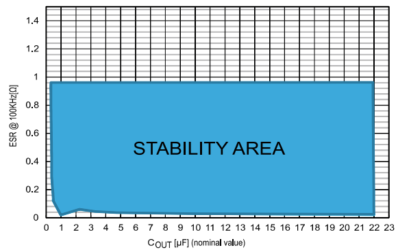
Figure 17: Stability area vs. (COUT, ESR)
