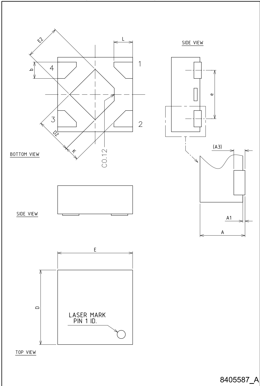
Figure 28: DFN4 1x1 package outline
