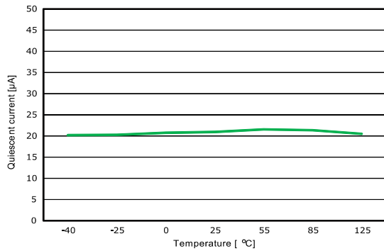
Figure 8: Quiescent current vs. temperature ( I_{OUT} = 0 \text{ mA} )
