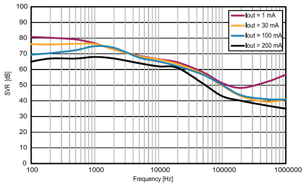
Figure 14: Supply voltage rejection vs. frequency
