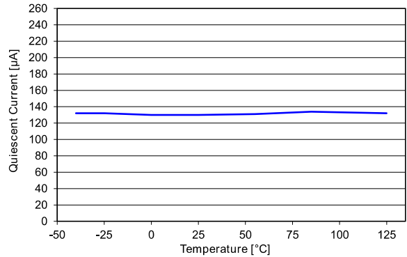
Figure 9: Quiescent current vs. temperature ( I_{OUT} = 200 \text{ mA} )
