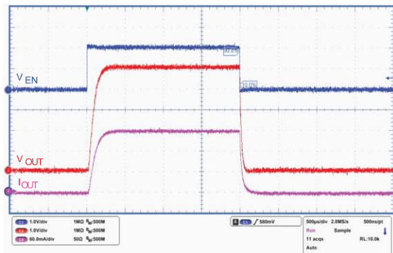
Figure 19: Enable startup ( V_{OUT} = 5\text{ V} )
