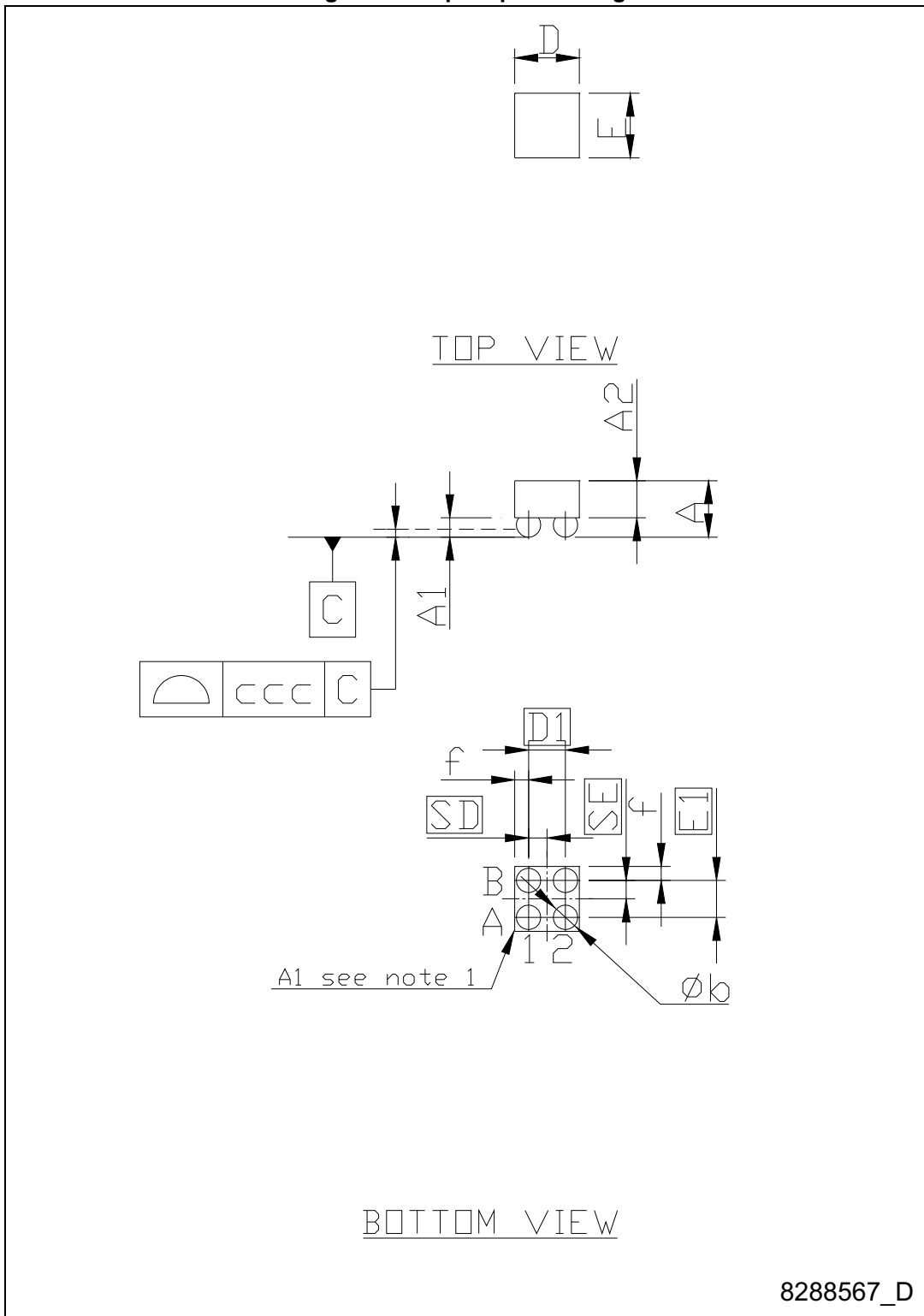
Figure 47. Flip-chip 4 drawing
