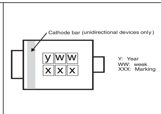
Figure 12. Marking information
